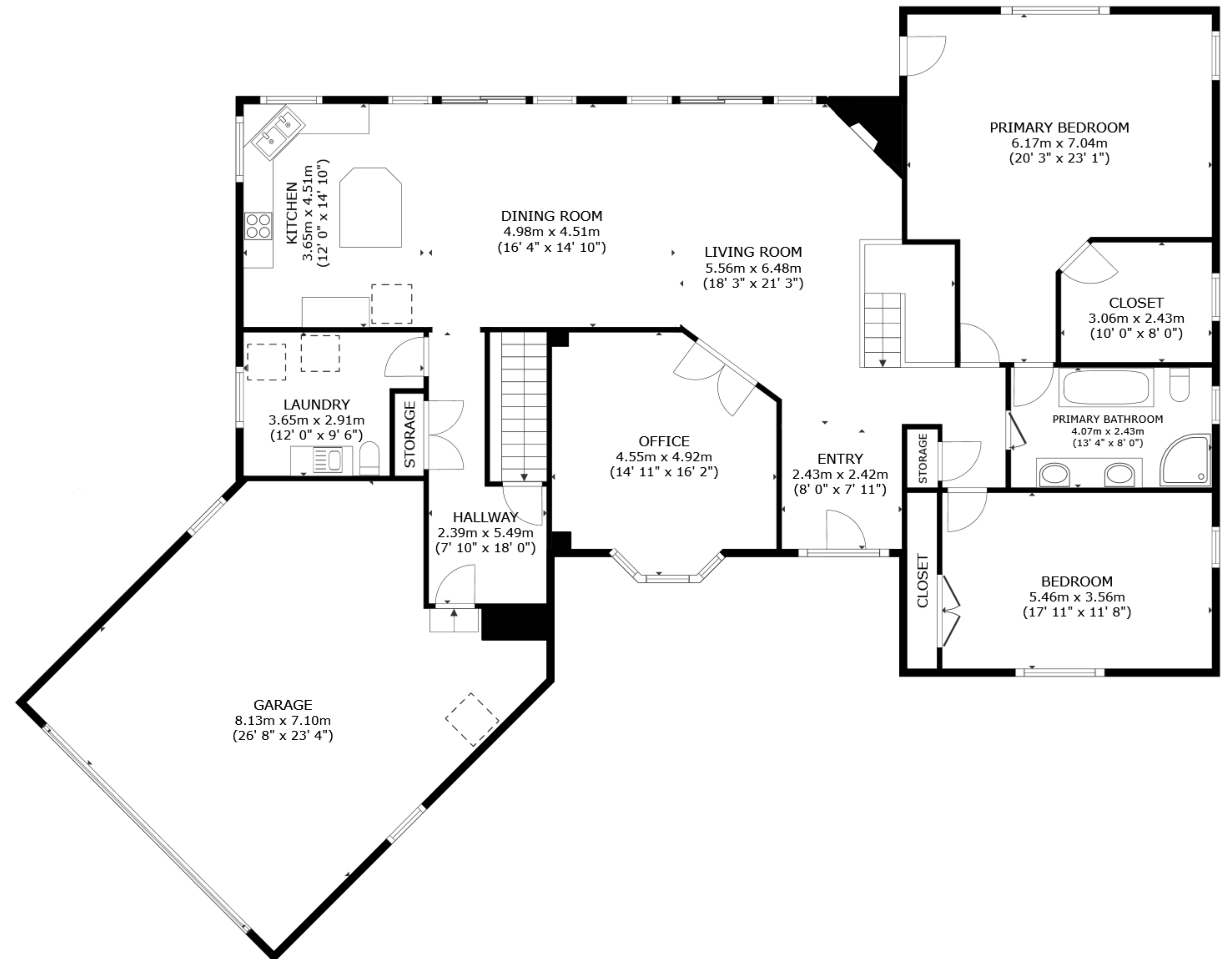
FLOOR 2
